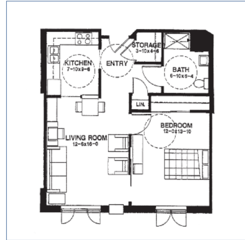
UNIT D handicap- accessible
